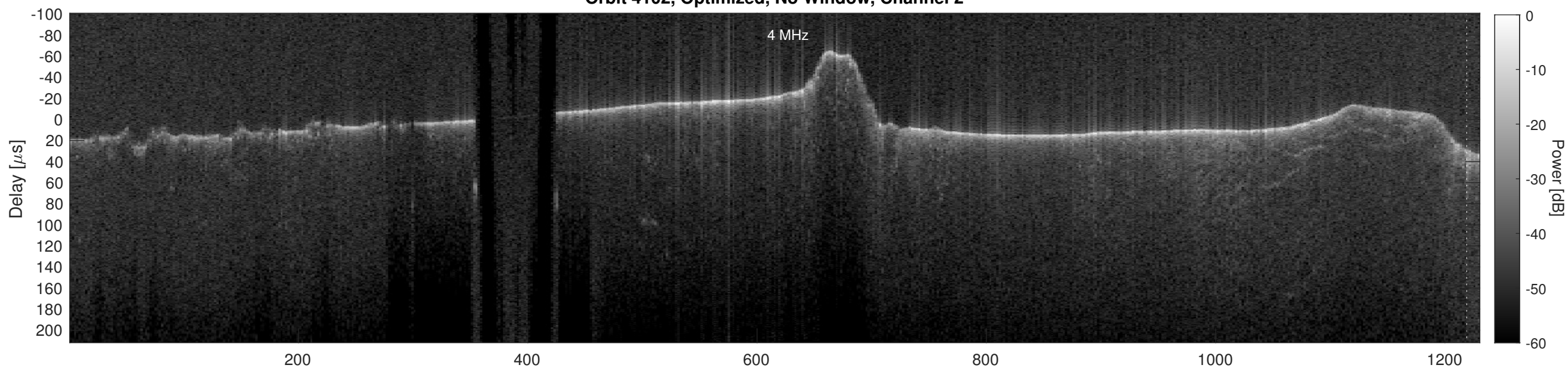
Orbit 4102, Cluttergram
