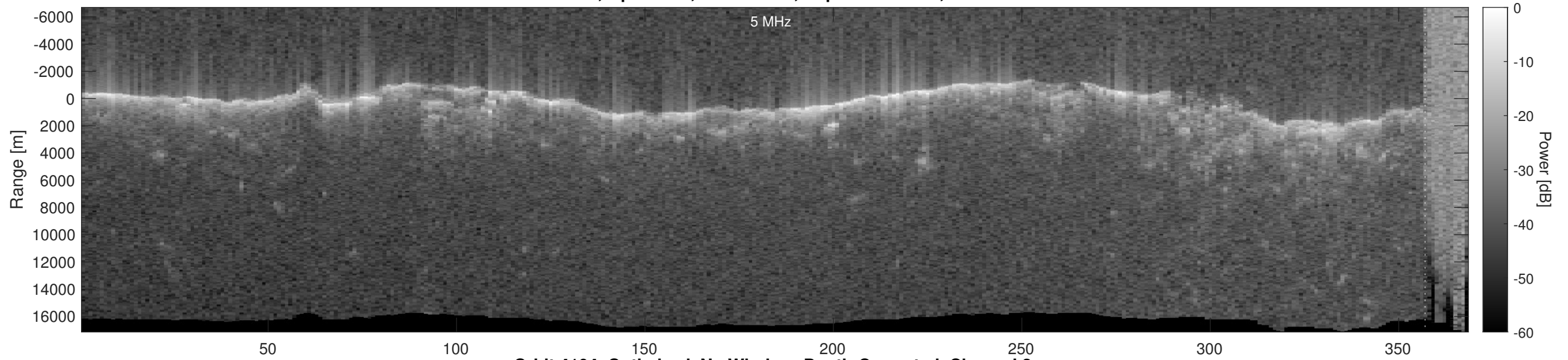
Orbit 4104, Optimized, No Window, Depth-Corrected, Channel 2
