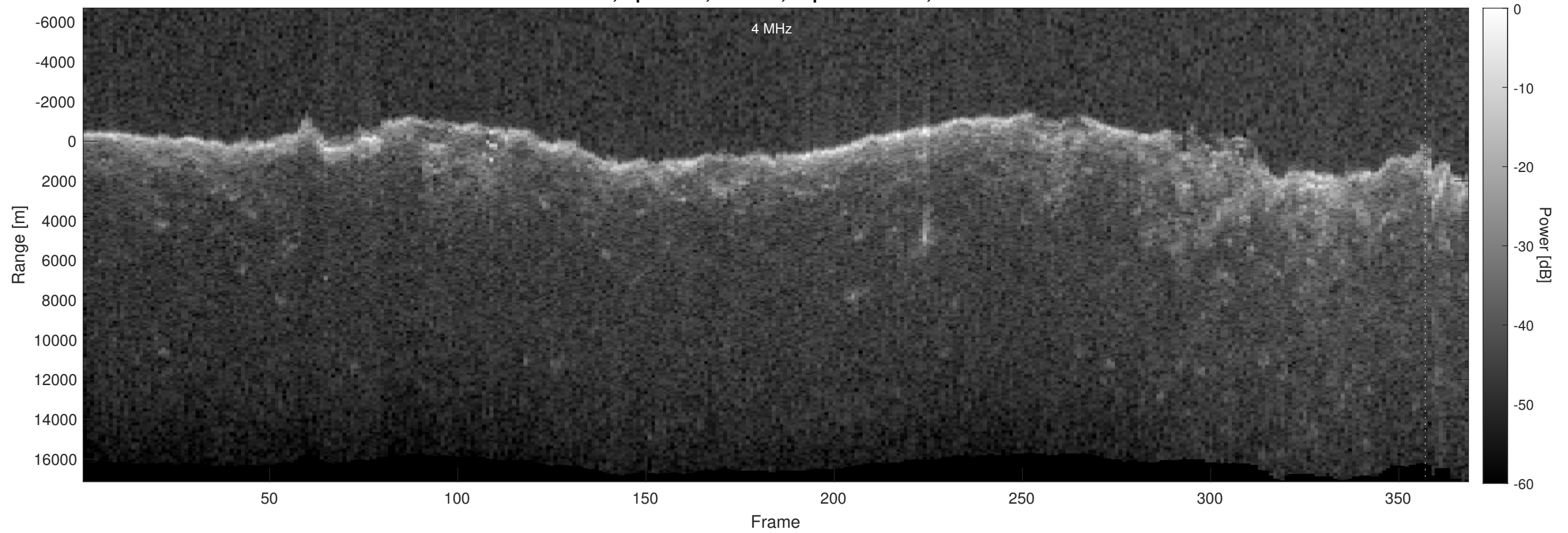
Orbit 4104, Optimized, Window, Depth-Corrected, Channel 2
