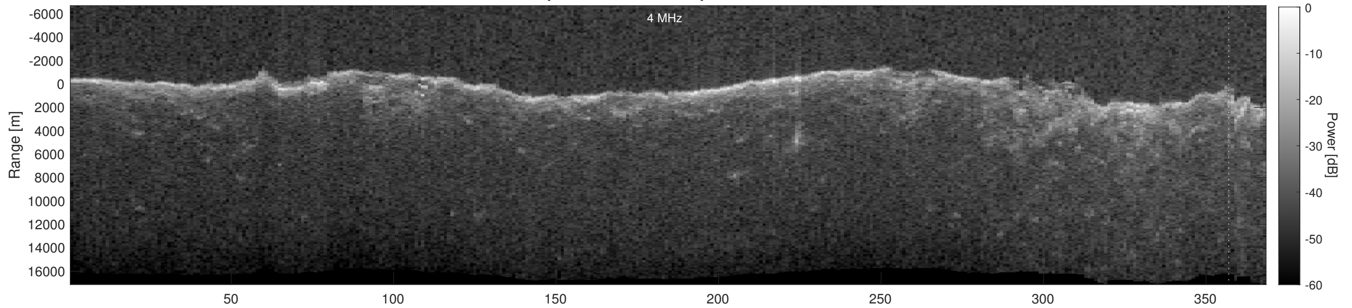
Orbit 4104, Depth-Corrected Cluttergram
