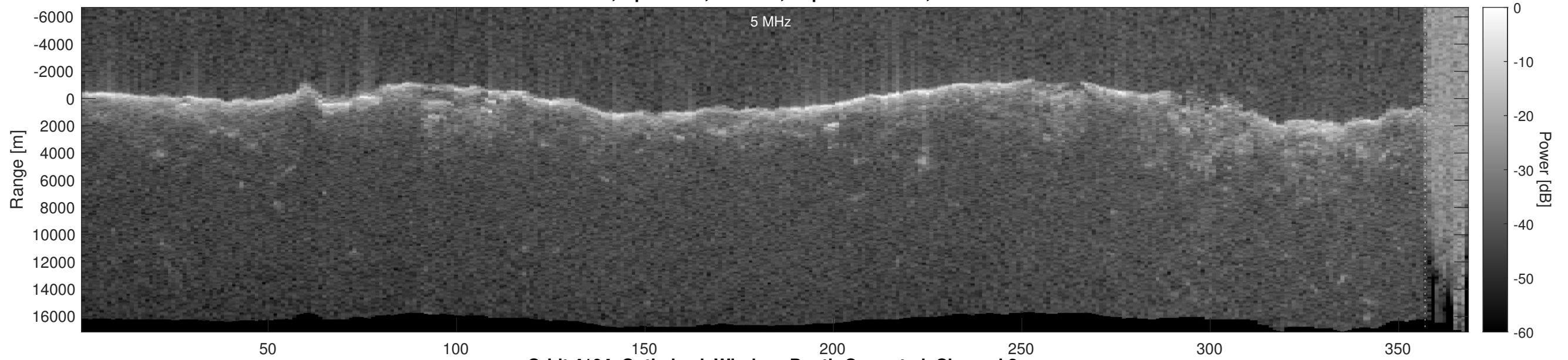
Orbit 4104, Optimized, Window, Depth-Corrected, Channel 2
