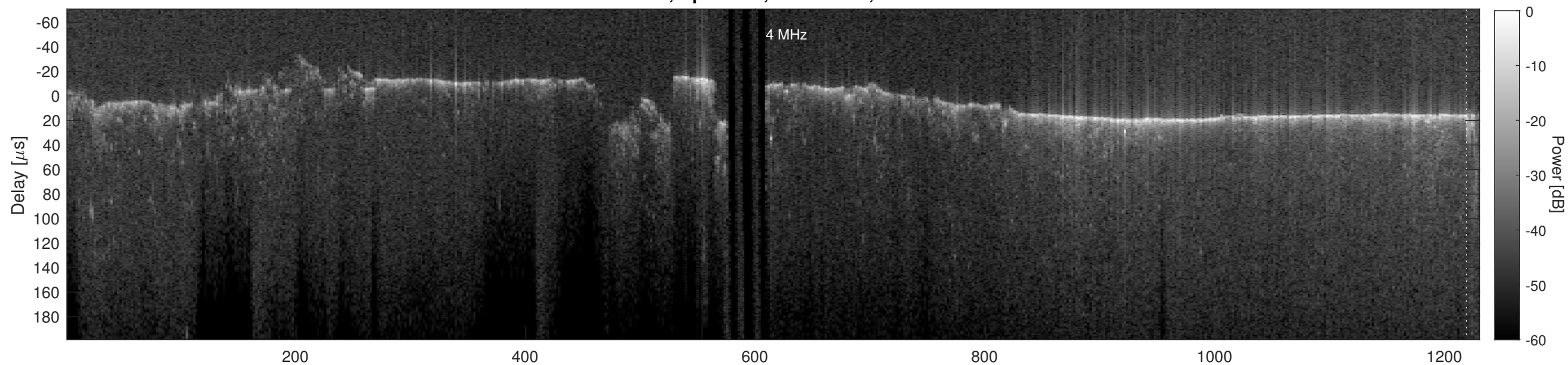
Orbit 4105, Cluttergram
