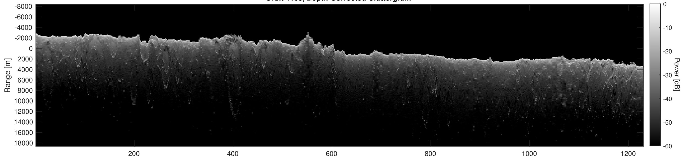
Orbit 4108, Depth-Corrected Cluttergram
