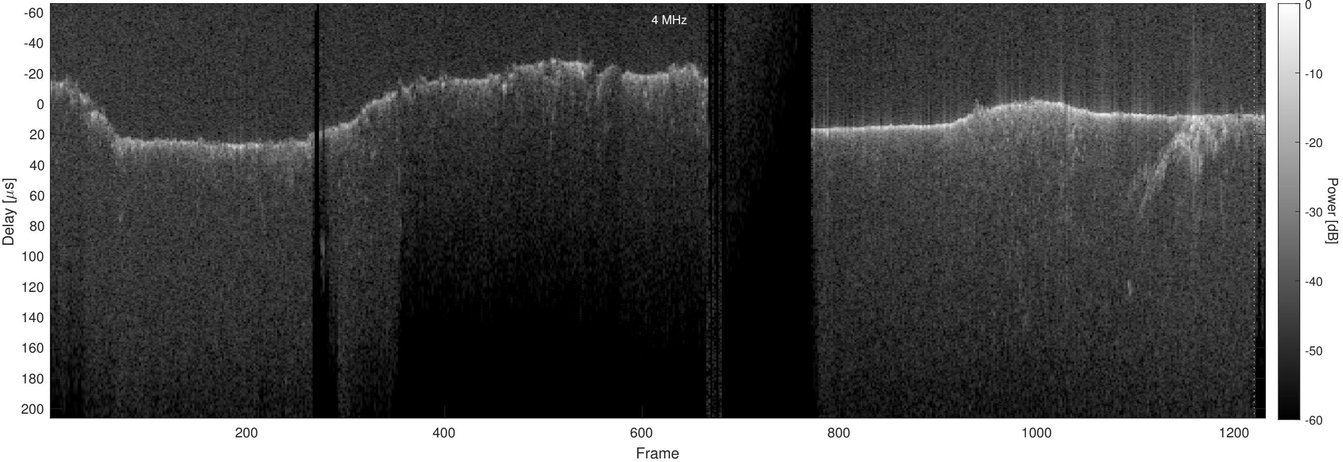
Orbit 4111, Optimized, No Window, Channel 2
