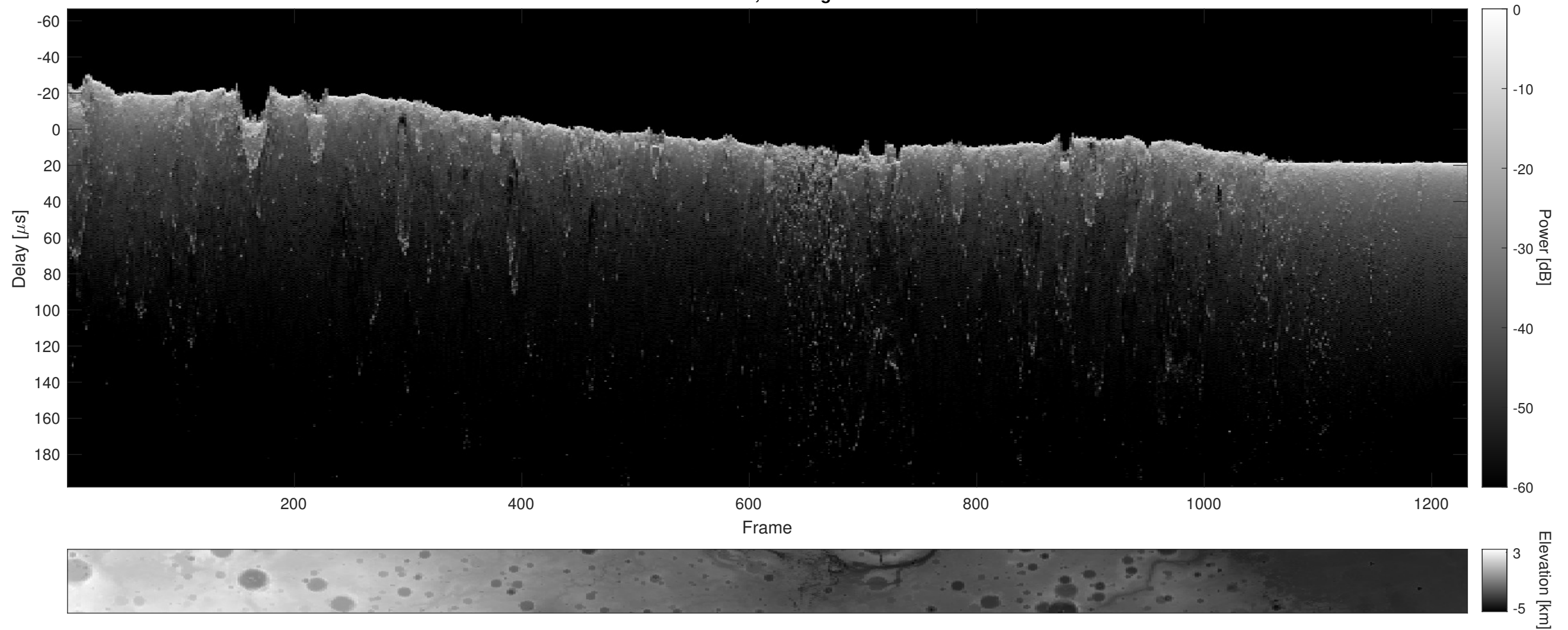
Orbit 4112, Cluttergram
