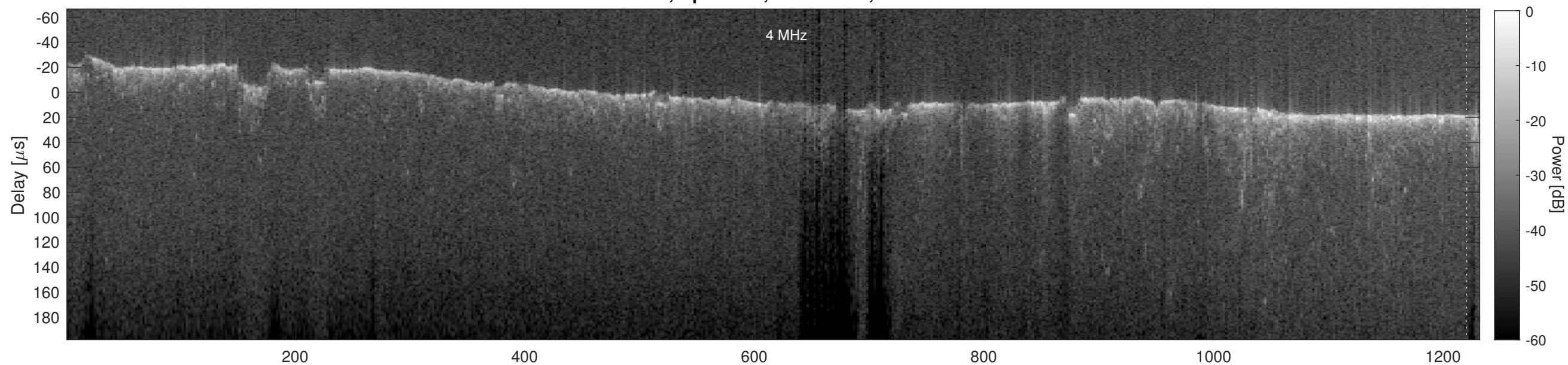
Orbit 4112, Cluttergram
