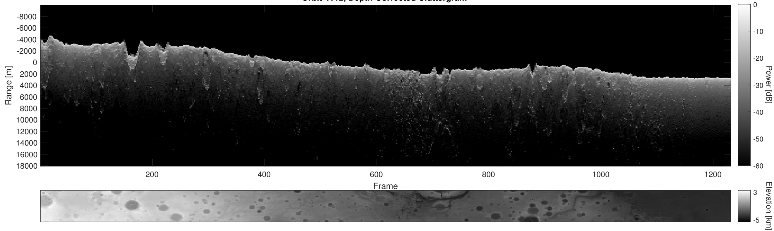
Orbit 4112, Depth-Corrected Cluttergram
