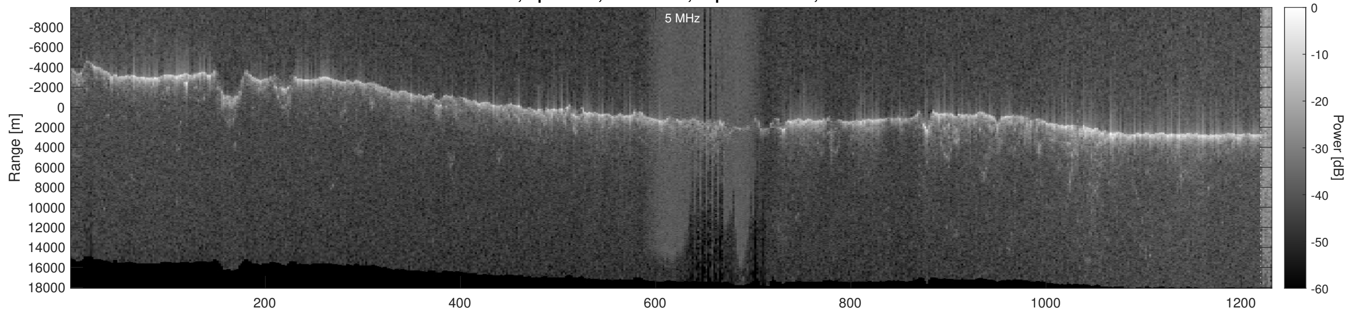
Orbit 4112, Optimized, No Window, Depth-Corrected, Channel 2
