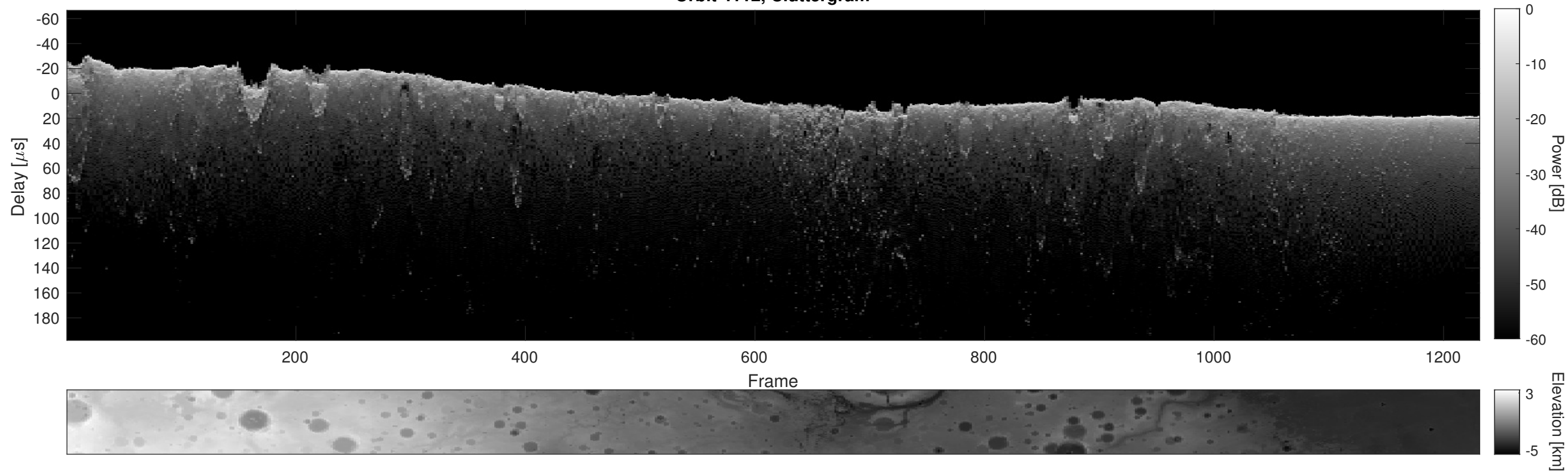
Orbit 4112, Cluttergram
