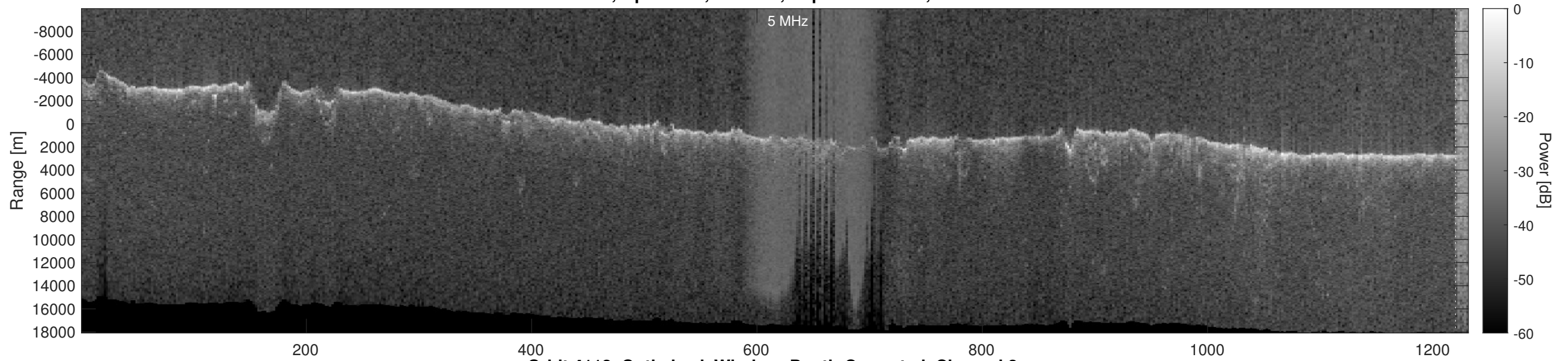
Orbit 4112, Optimized, Window, Depth-Corrected, Channel 2
