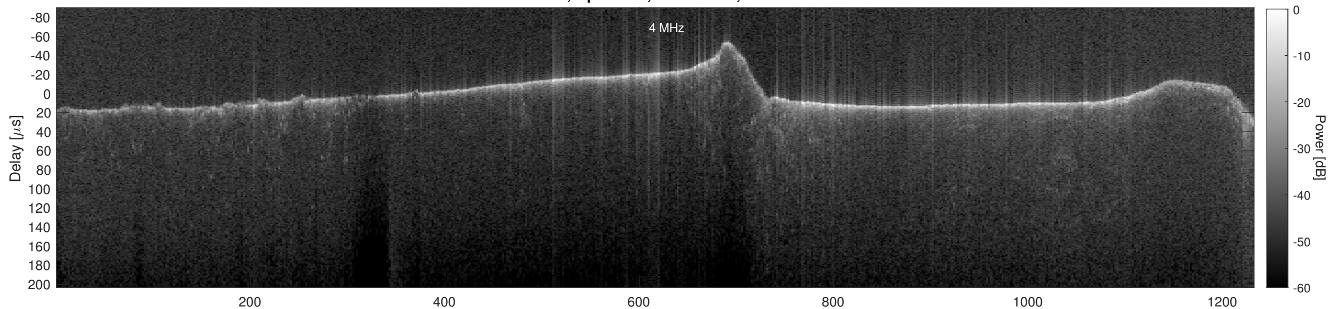
Orbit 4113, Cluttergram
