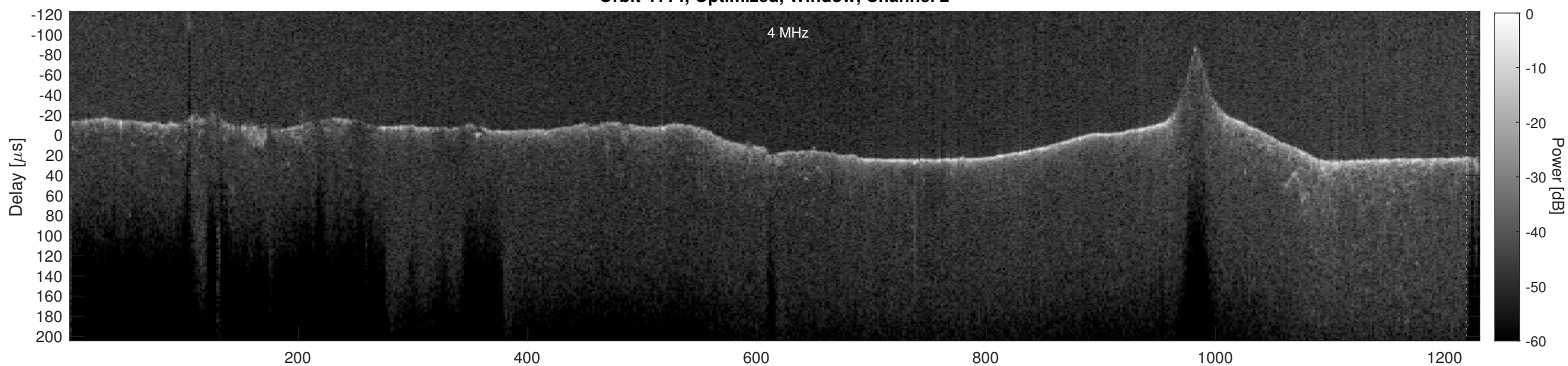
Orbit 4114, Cluttergram
