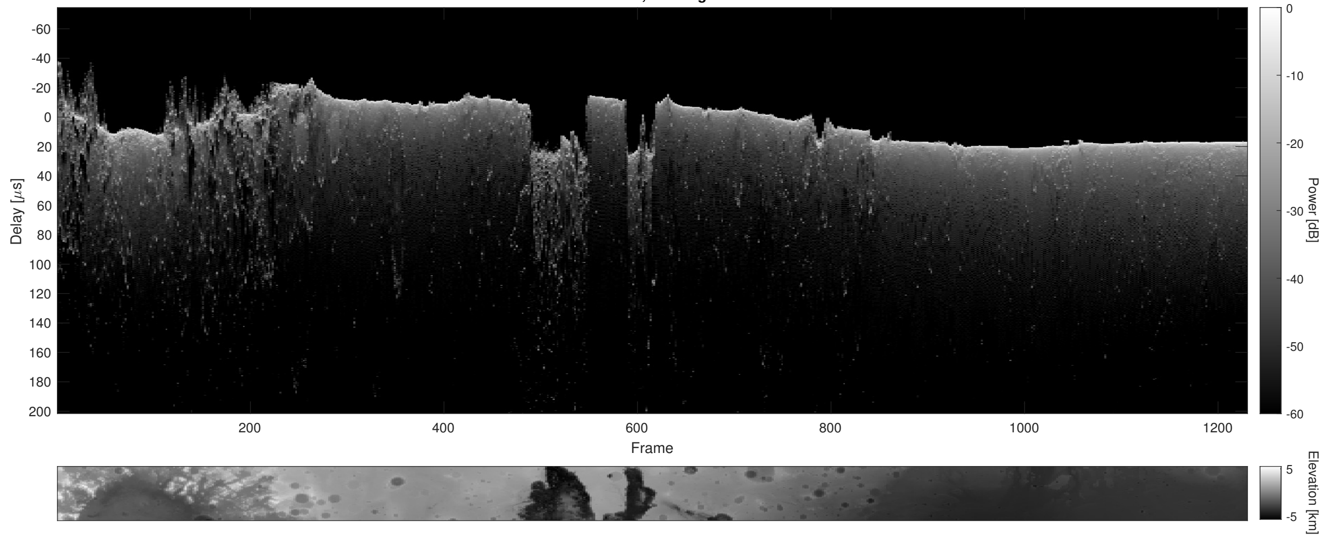
Orbit 4116, Cluttergram
