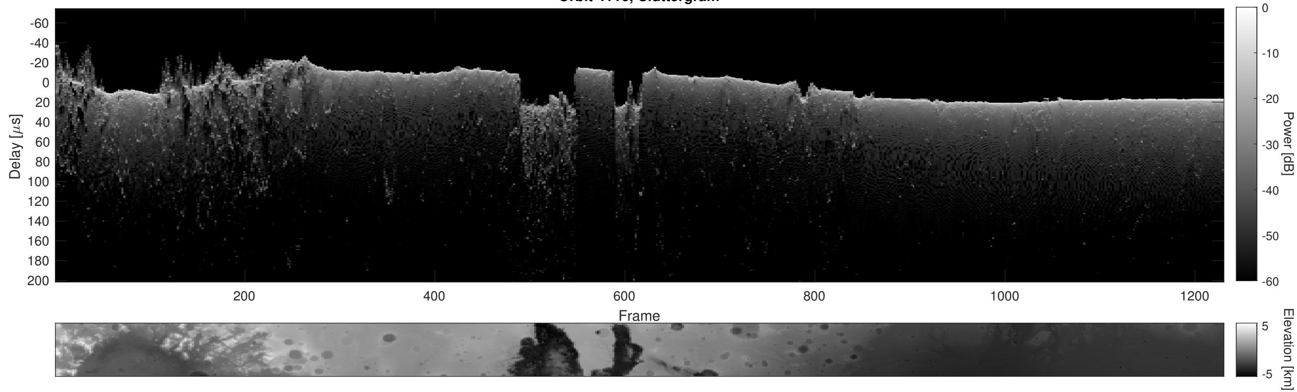
Orbit 4116, Cluttergram
