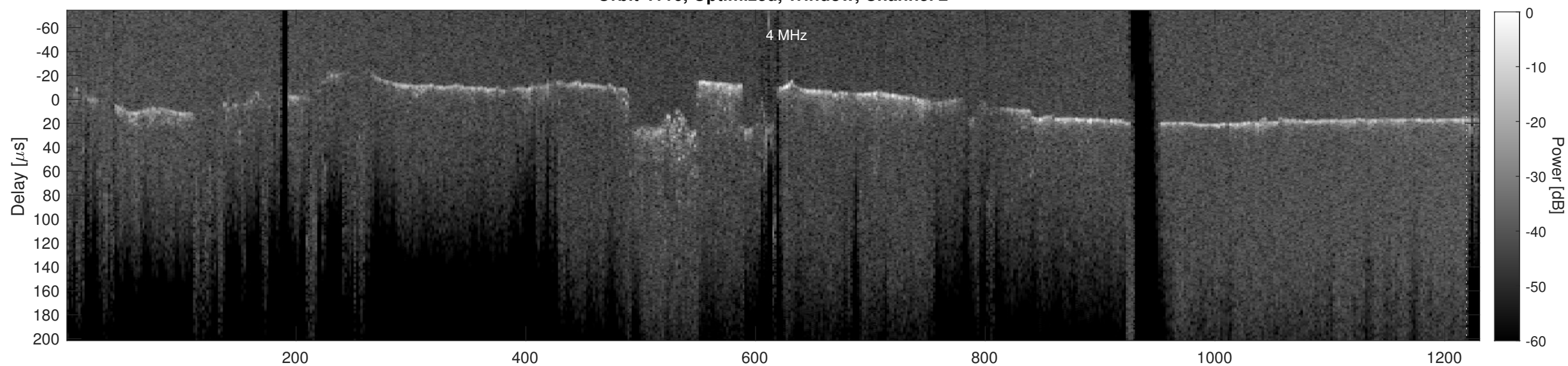
Orbit 4116, Cluttergram
