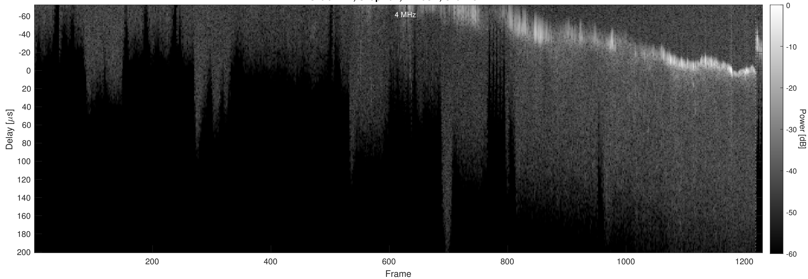
Orbit 4117, Chapman, Window, Channel 2
