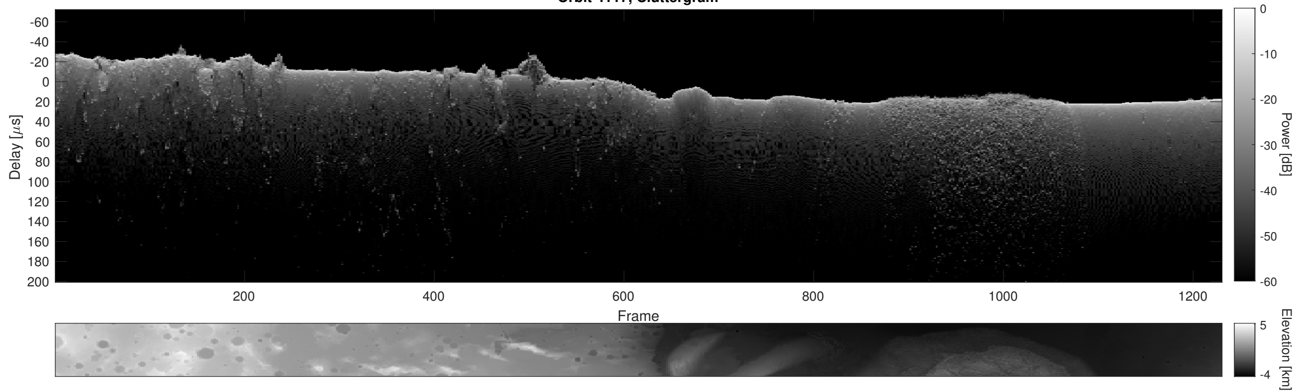
Orbit 4117, Cluttergram
