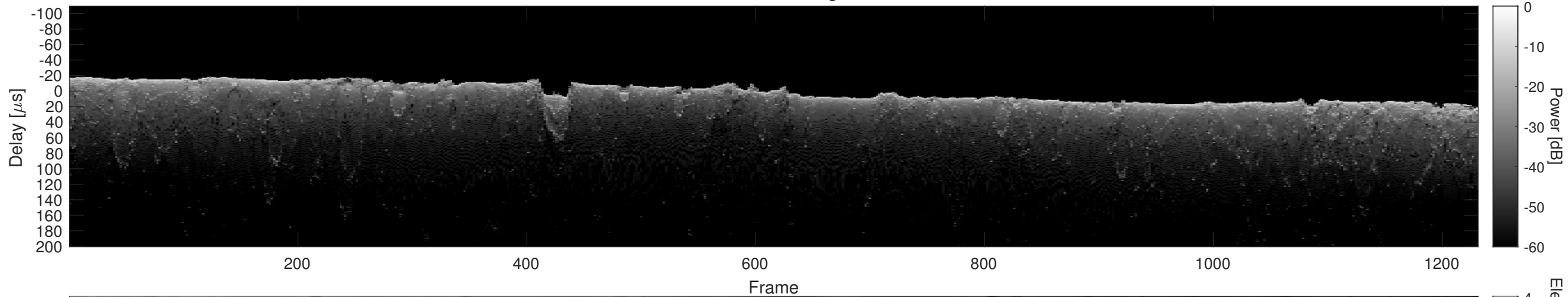
Orbit 4119, Cluttergram
