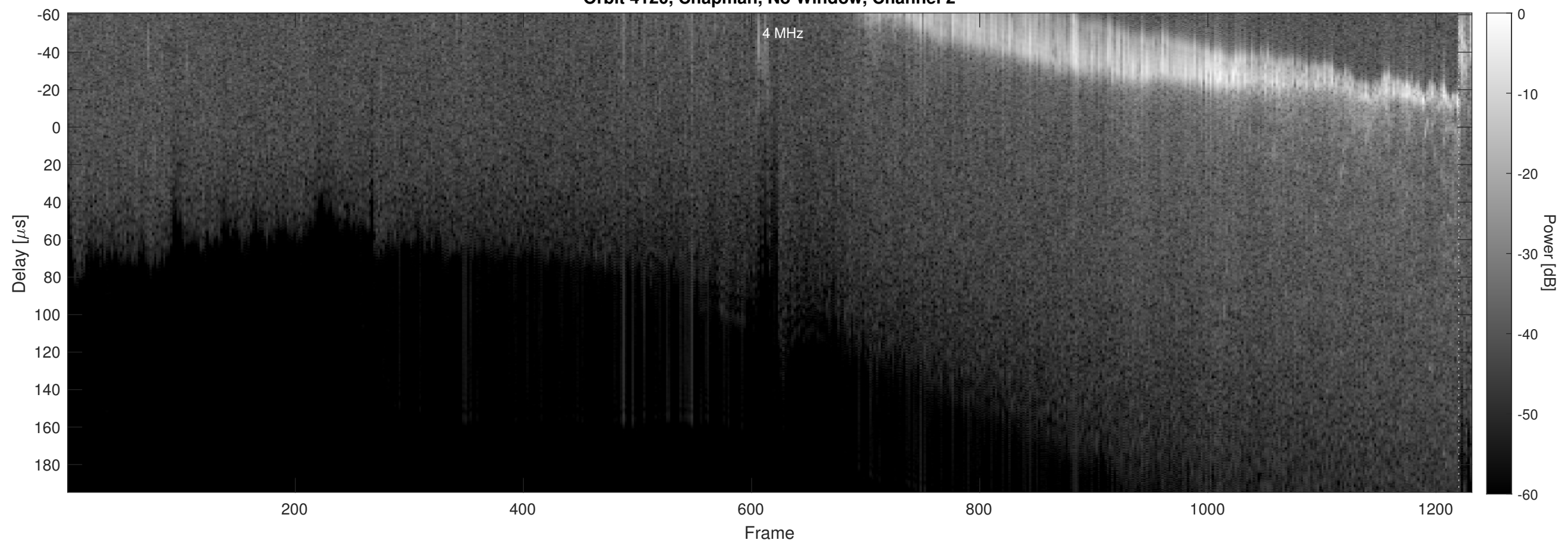
Orbit 4120, Chapman, No Window, Channel 2
