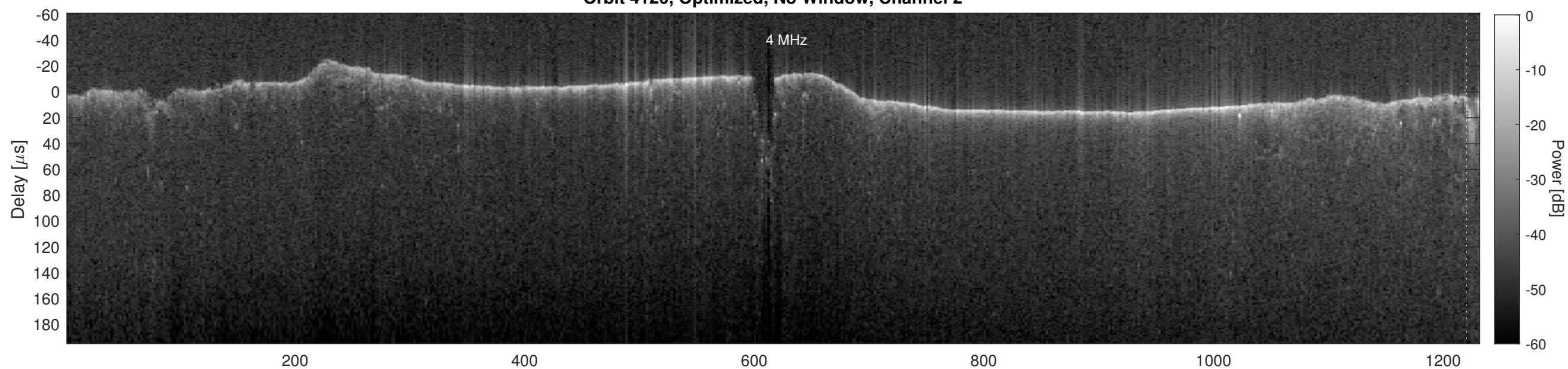
Orbit 4120, Cluttergram
