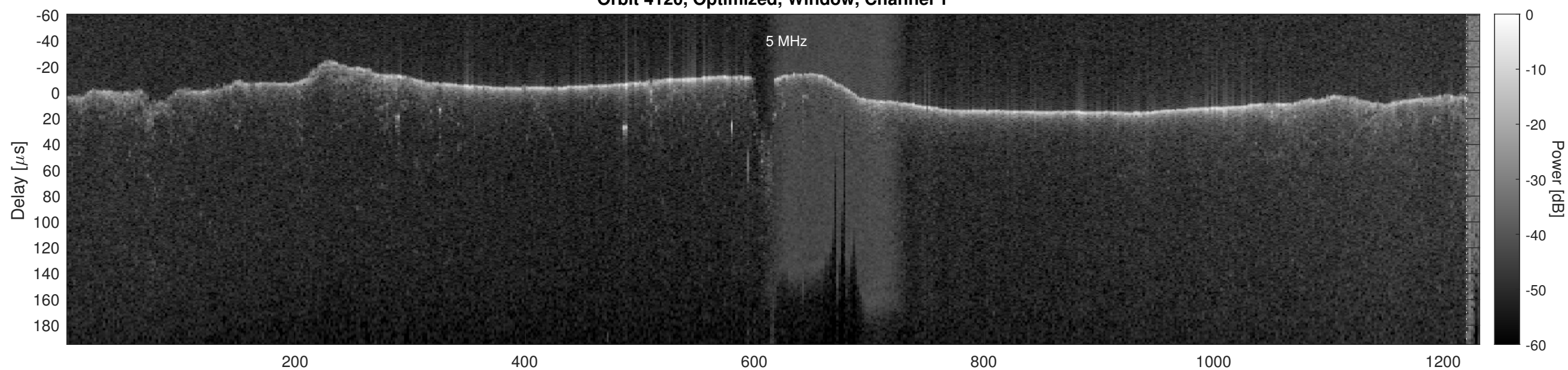
Orbit 4120, Optimized, Window, Channel 2
