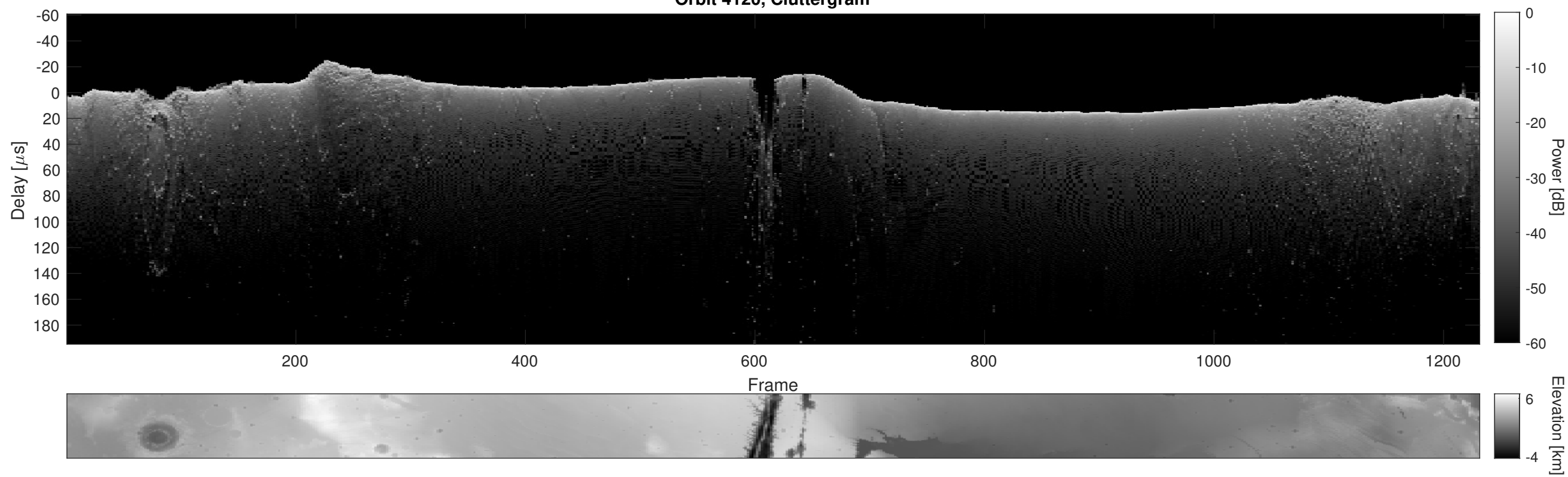
Orbit 4120, Cluttergram
