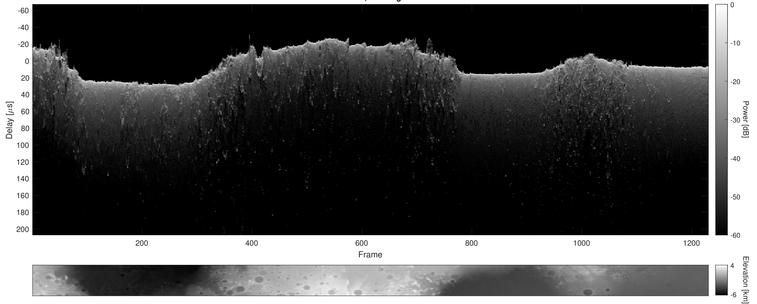
Orbit 4122, Cluttergram
