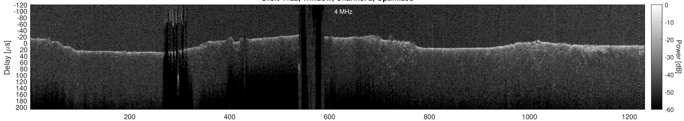
Orbit 4122, Cluttergram
