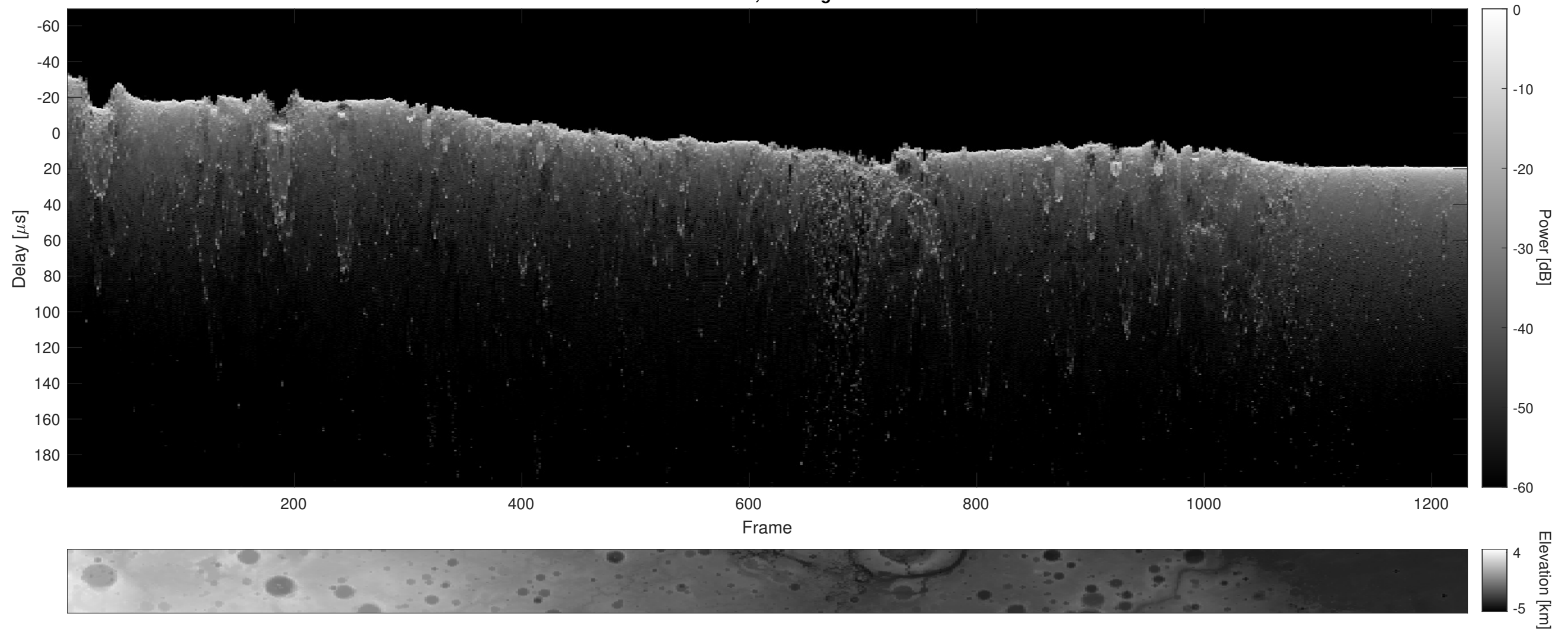
Orbit 4123, Cluttergram
