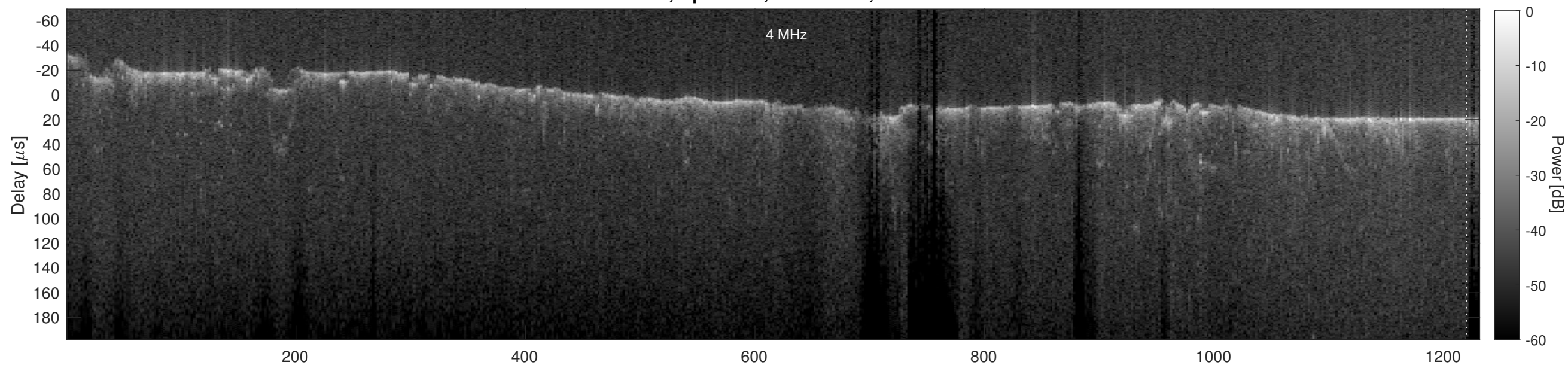
Orbit 4123, Cluttergram
