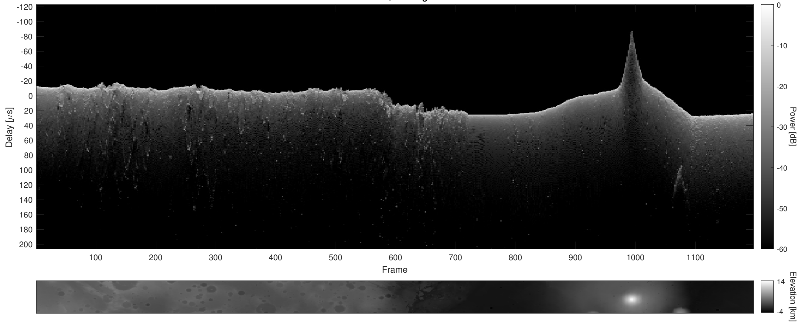
Orbit 4125, Cluttergram
