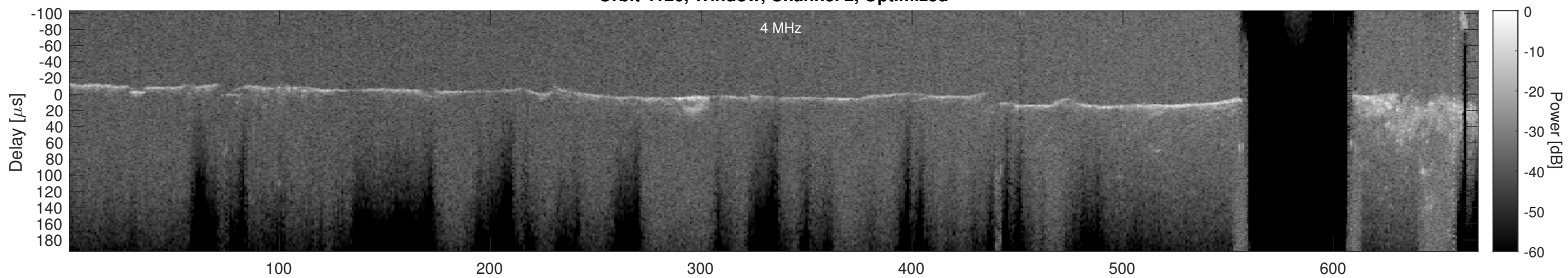
Orbit 4126, Cluttergram
