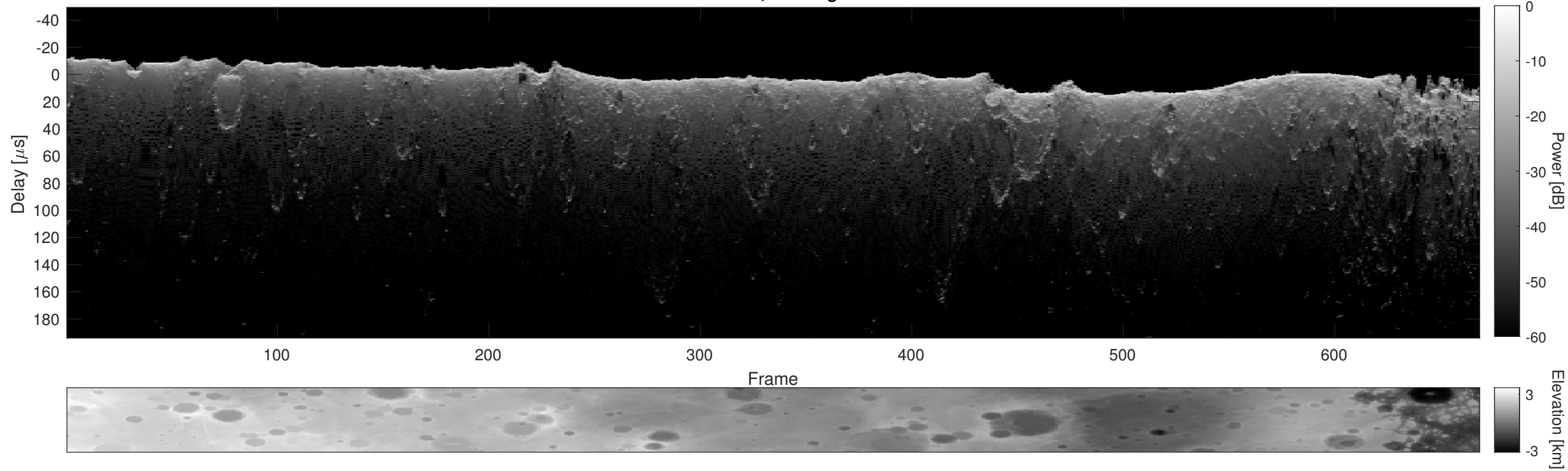
Orbit 4126, Cluttergram
