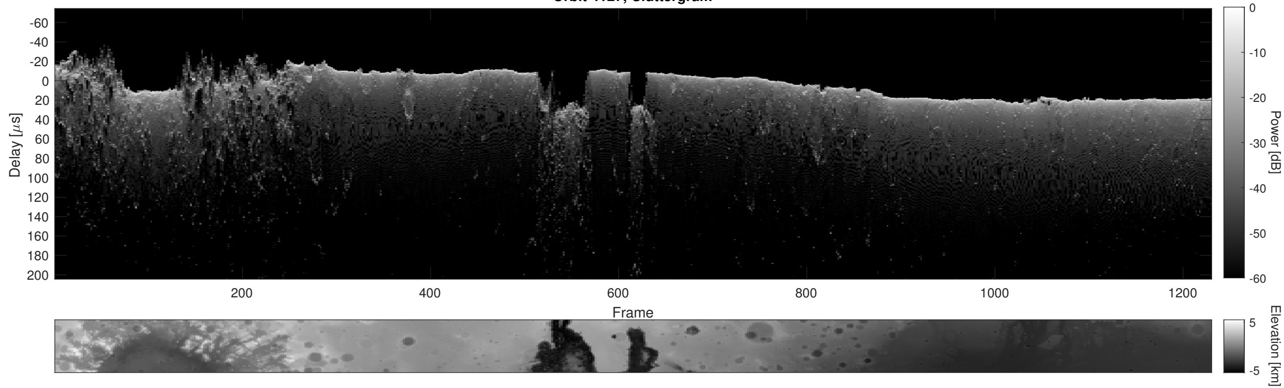
Orbit 4127, Cluttergram
