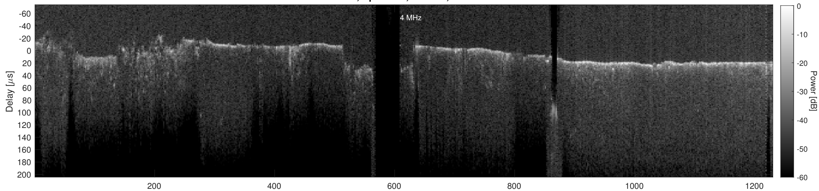
Orbit 4127, Cluttergram
