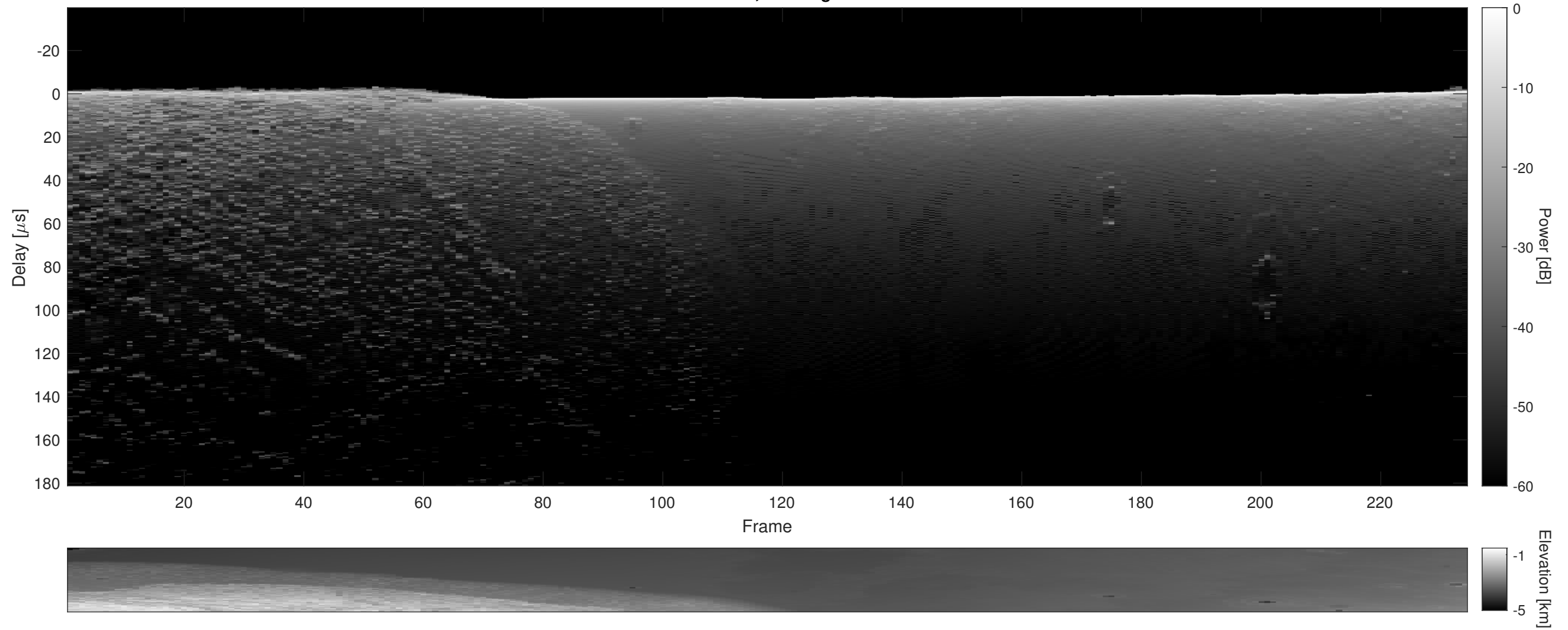
Orbit 4128, Cluttergram
