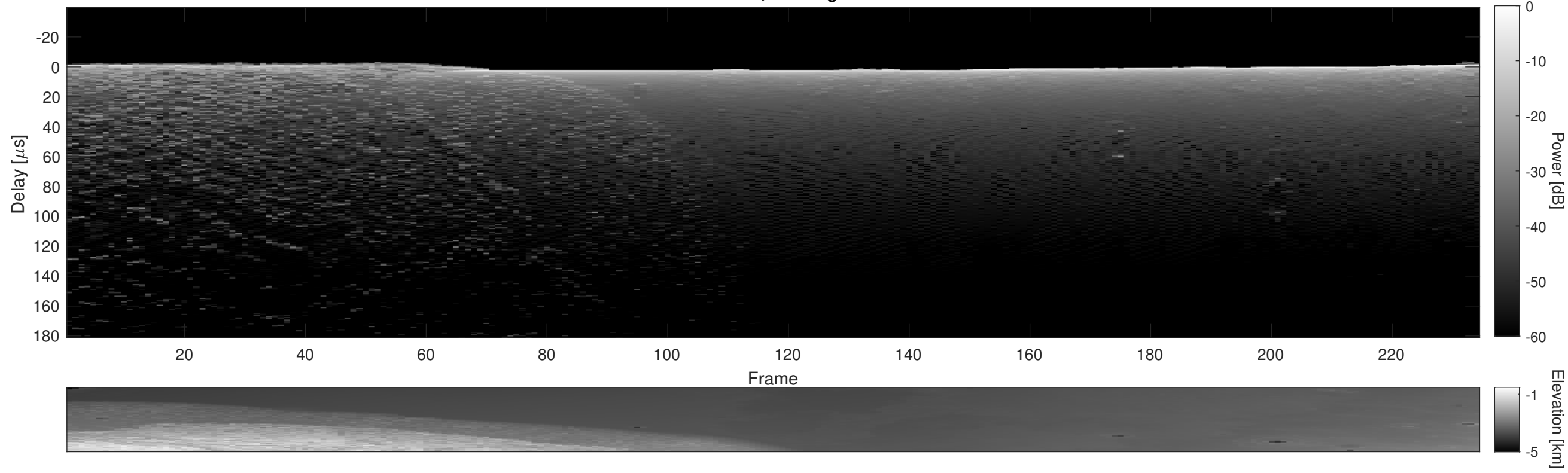
Orbit 4128, Cluttergram
