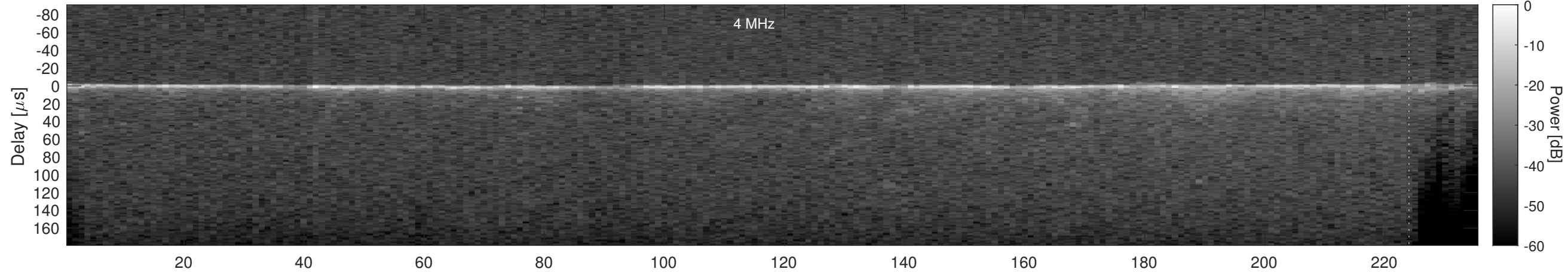
Orbit 4129, Cluttergram
