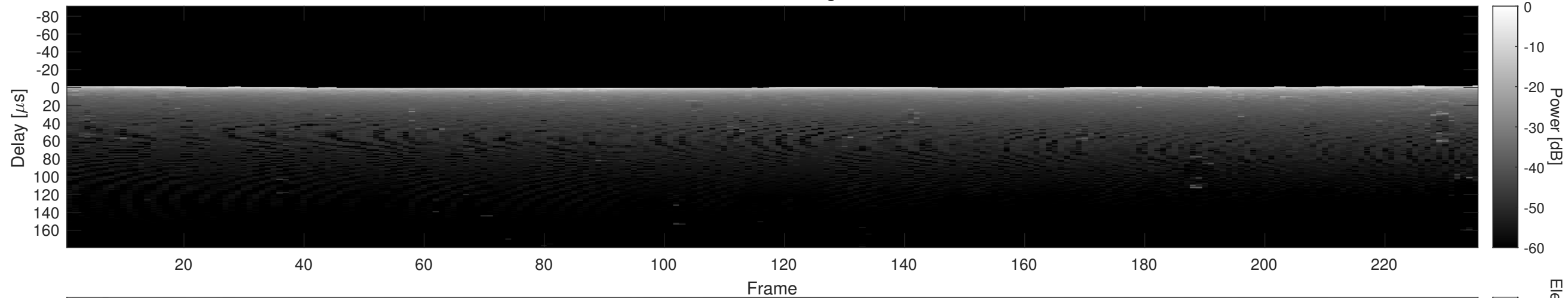
Orbit 4129, Cluttergram
