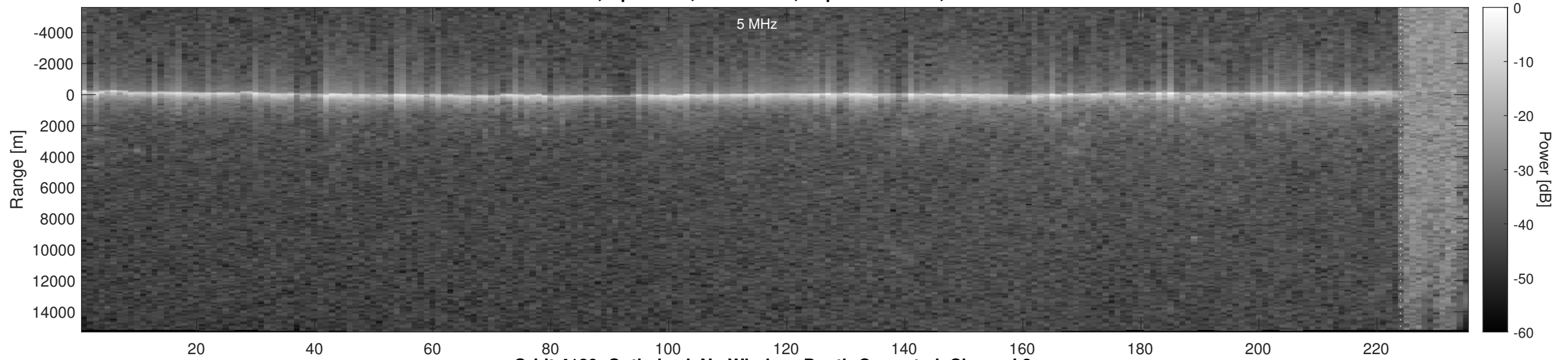
Orbit 4129, Optimized, No Window, Depth-Corrected, Channel 2
