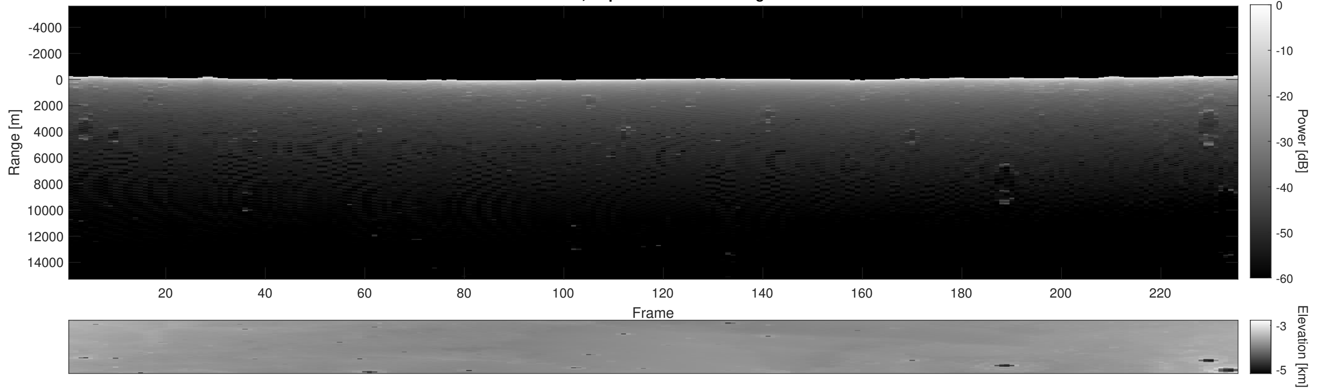
Orbit 4129, Depth-Corrected Cluttergram
