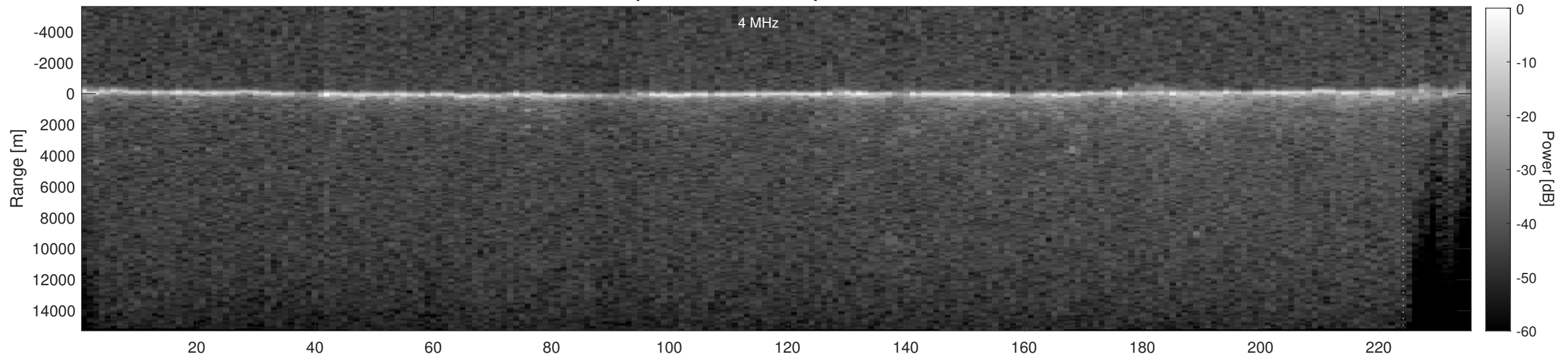
Orbit 4129, Depth-Corrected Cluttergram
