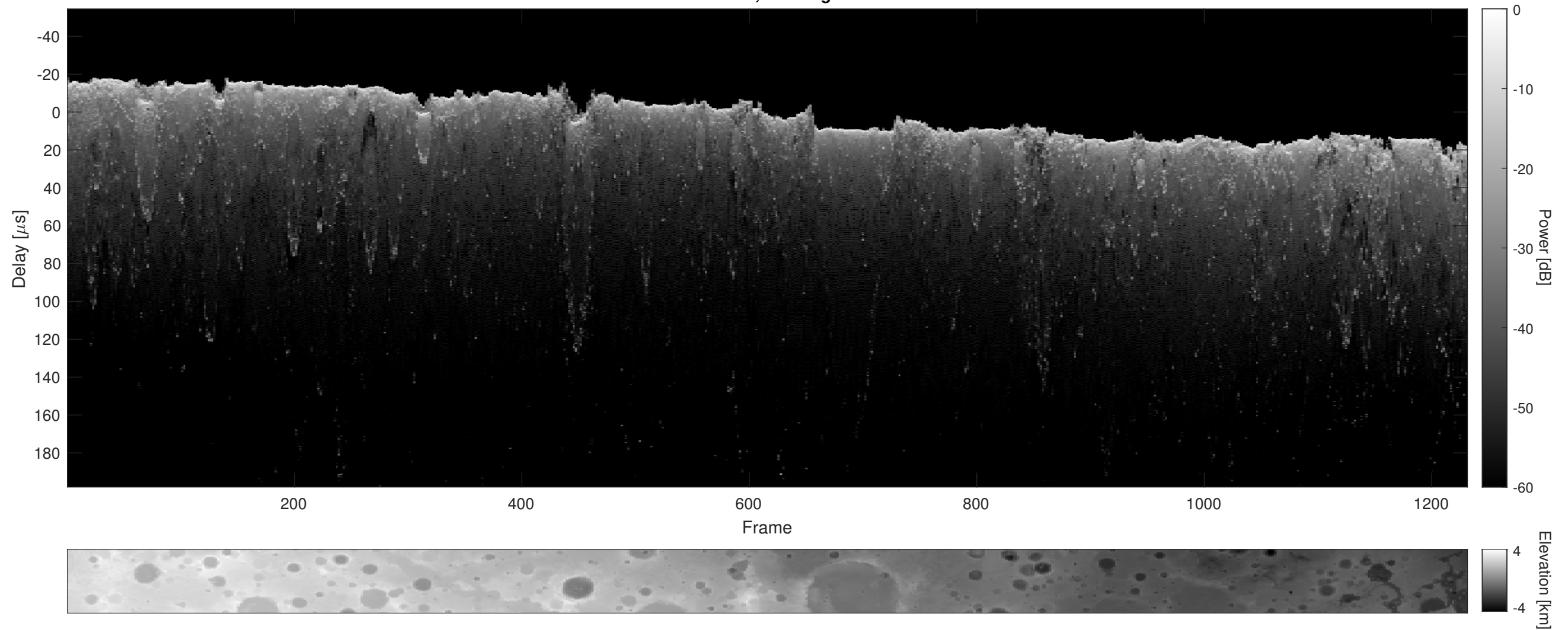
Orbit 4130, Cluttergram
