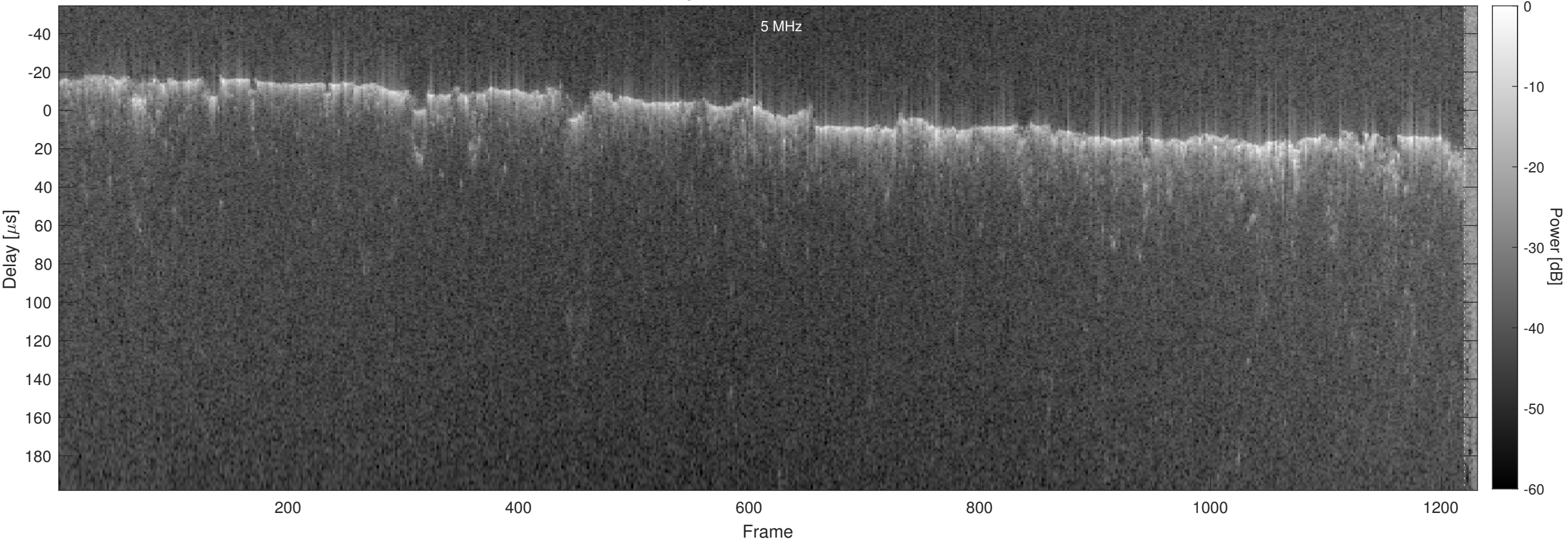
Orbit 4130, Optimized, No Window, Channel 2
