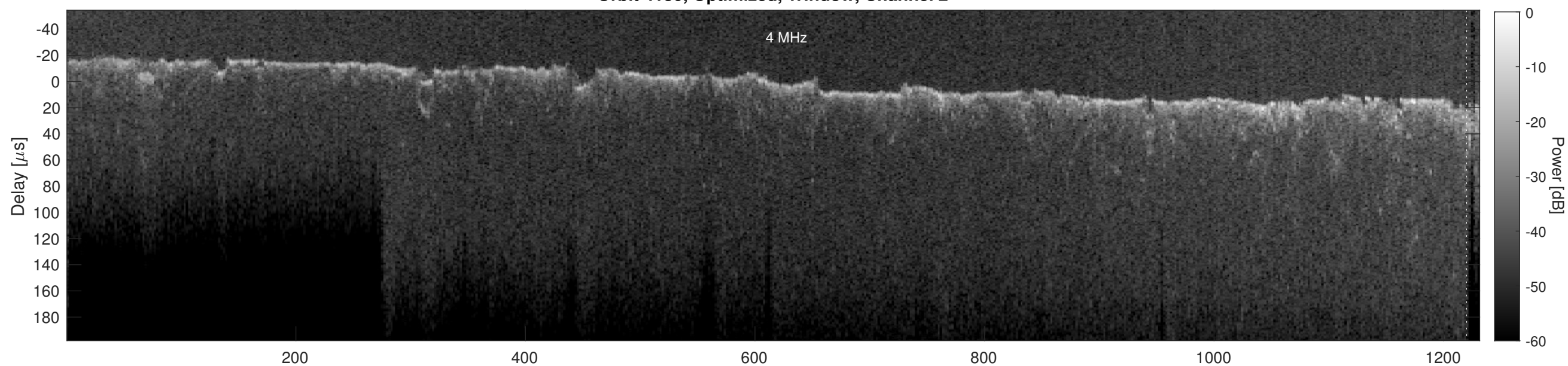
Orbit 4130, Cluttergram
