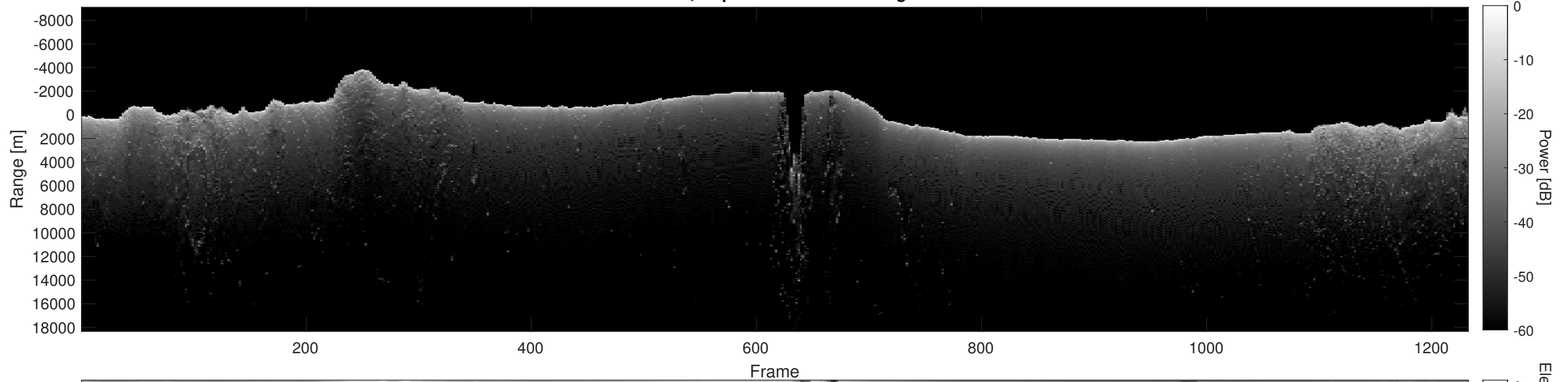
Orbit 4131, Depth-Corrected Cluttergram
