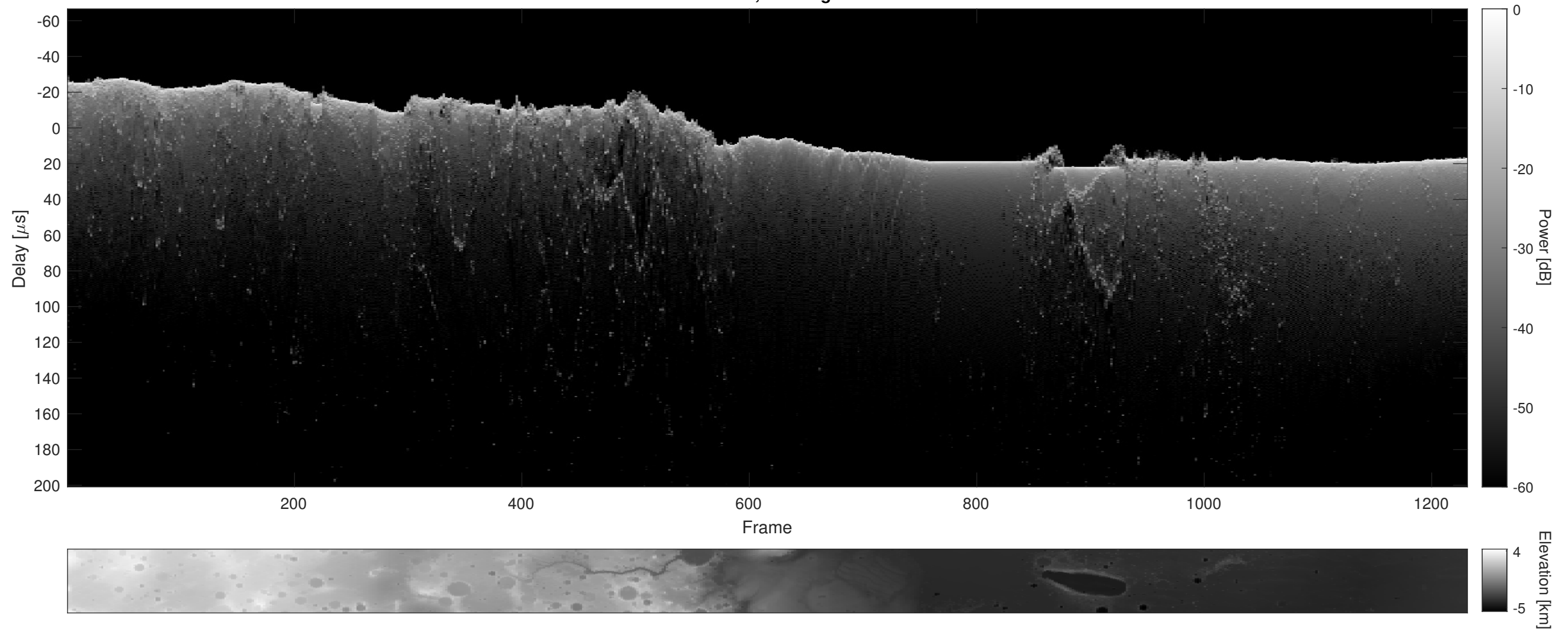
Orbit 4132, Cluttergram
