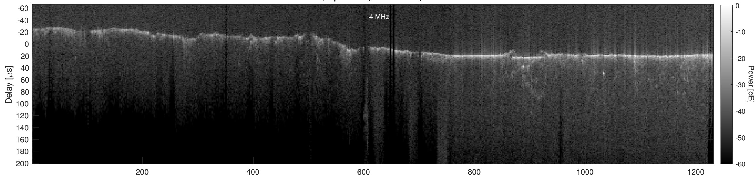
Orbit 4132, Cluttergram
