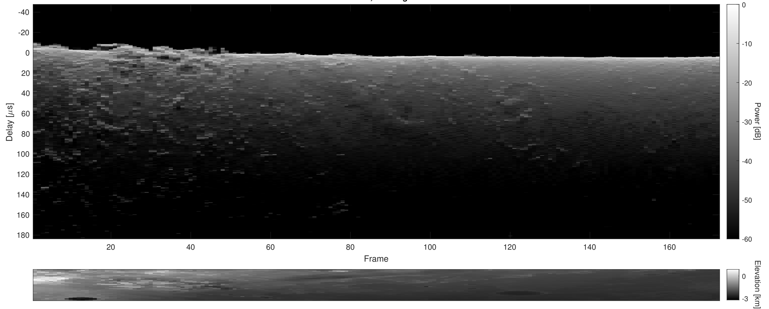
Orbit 4133, Cluttergram
