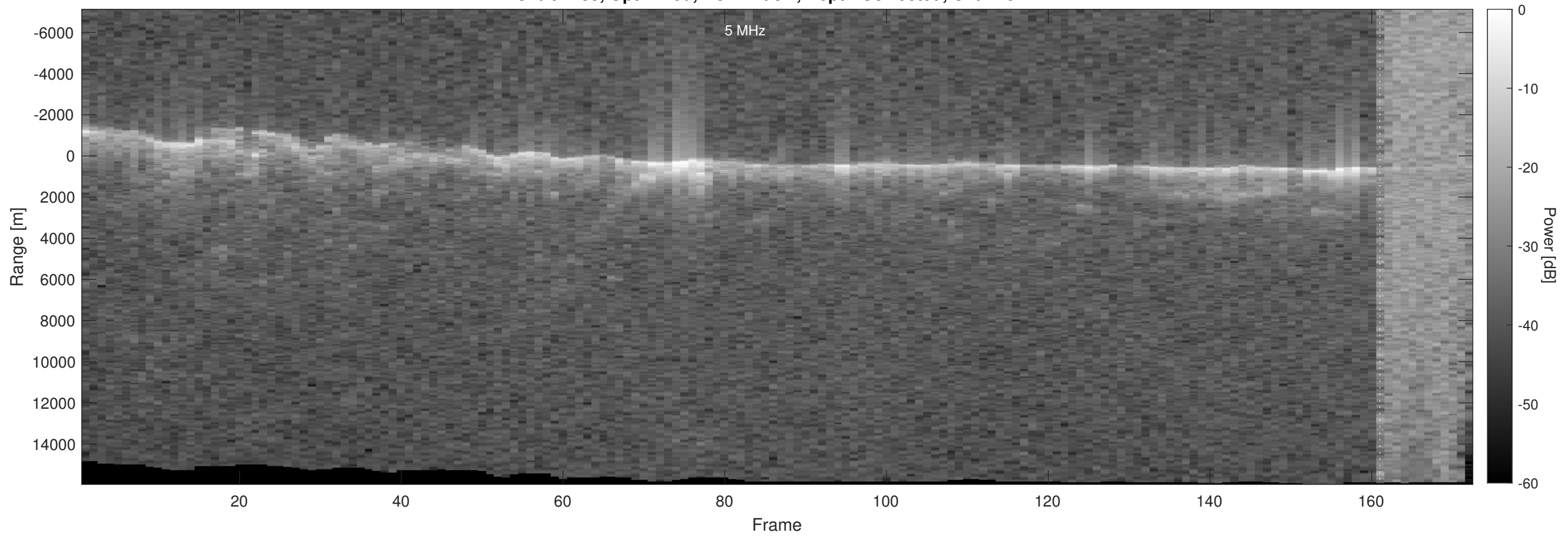
Orbit 4133, Optimized, No Window, Depth-Corrected, Channel 2
