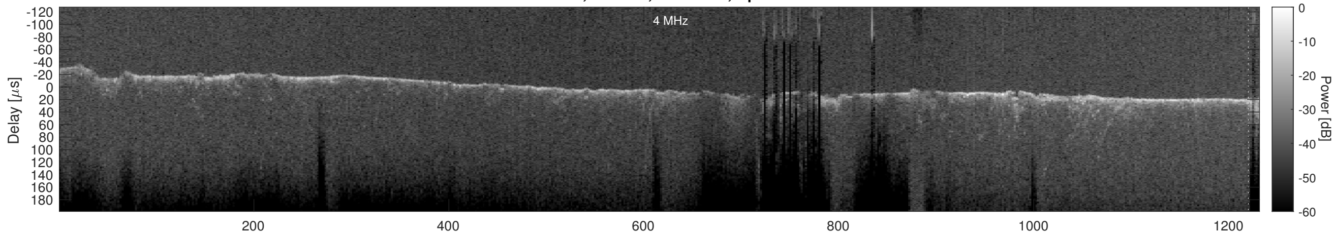
Orbit 4134, Cluttergram
