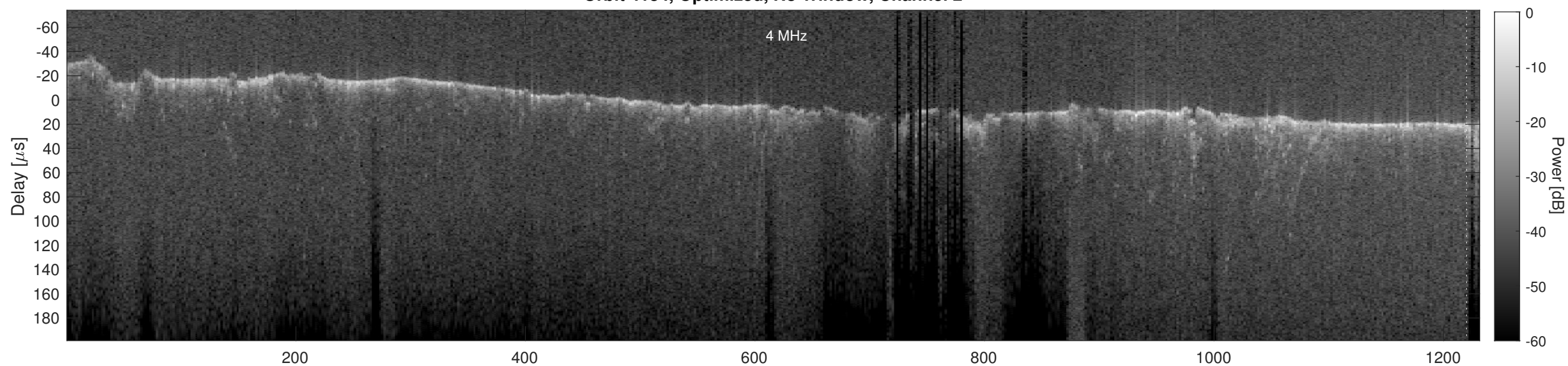
Orbit 4134, Cluttergram
