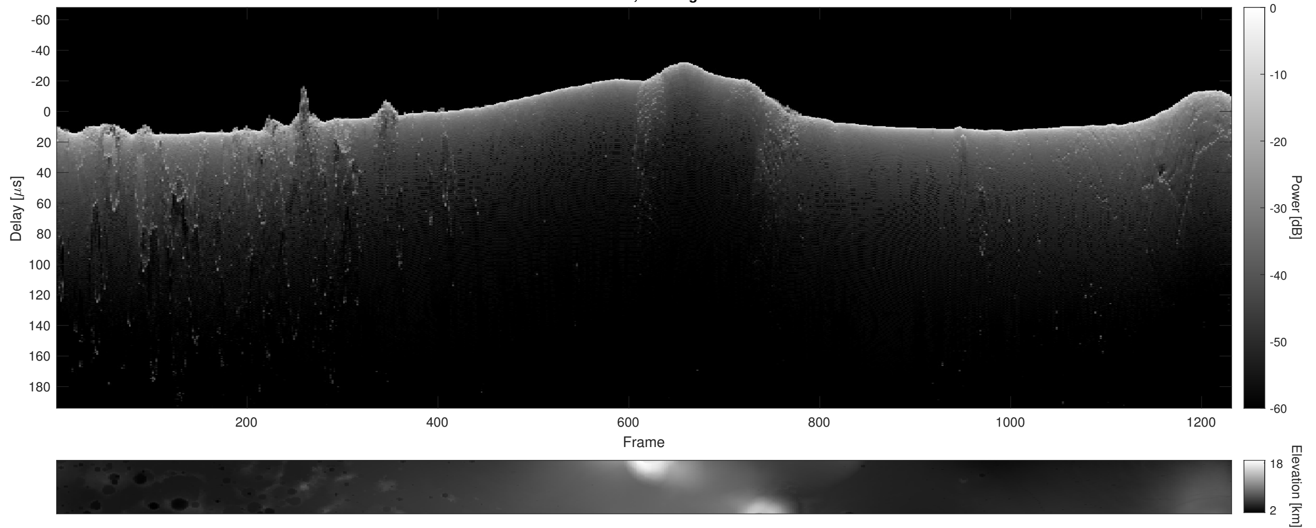
Orbit 4135, Cluttergram
