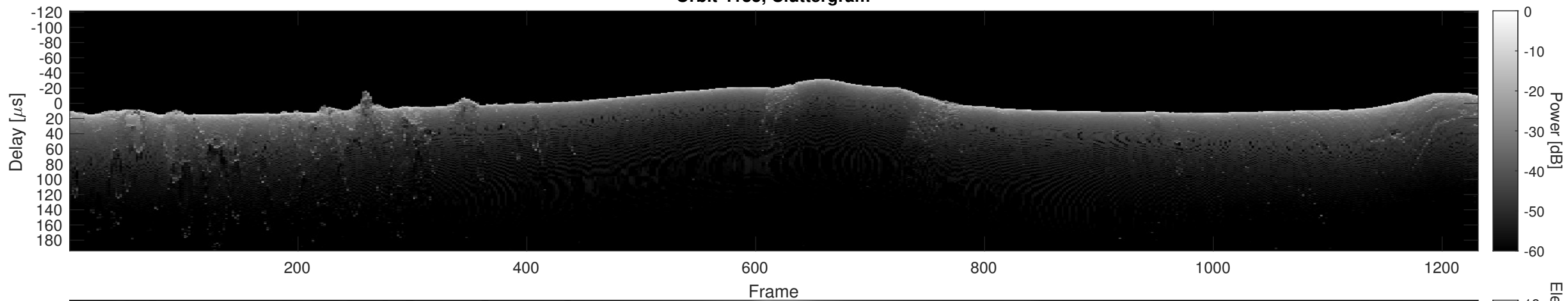
Orbit 4135, Cluttergram
