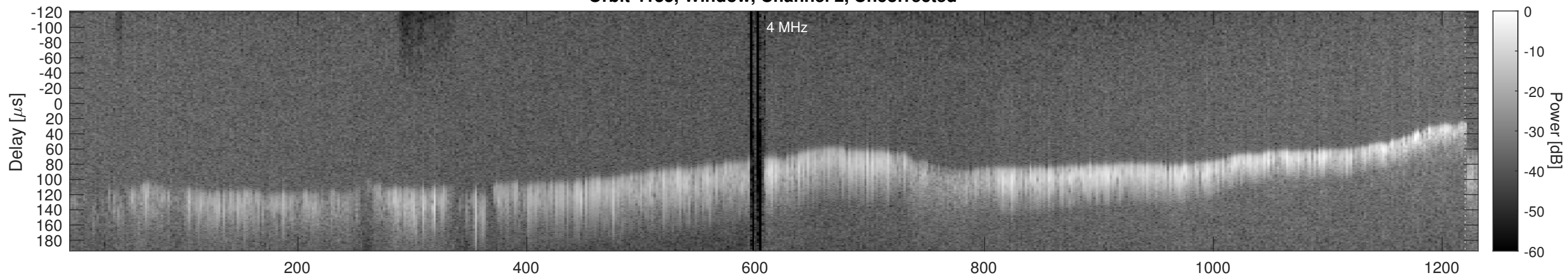
Orbit 4135, Window, Channel 2, Chapman
