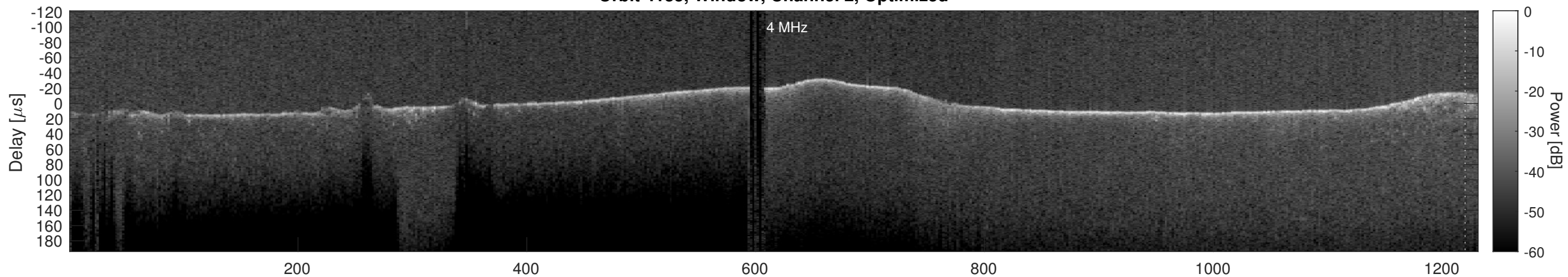
Orbit 4135, Cluttergram
