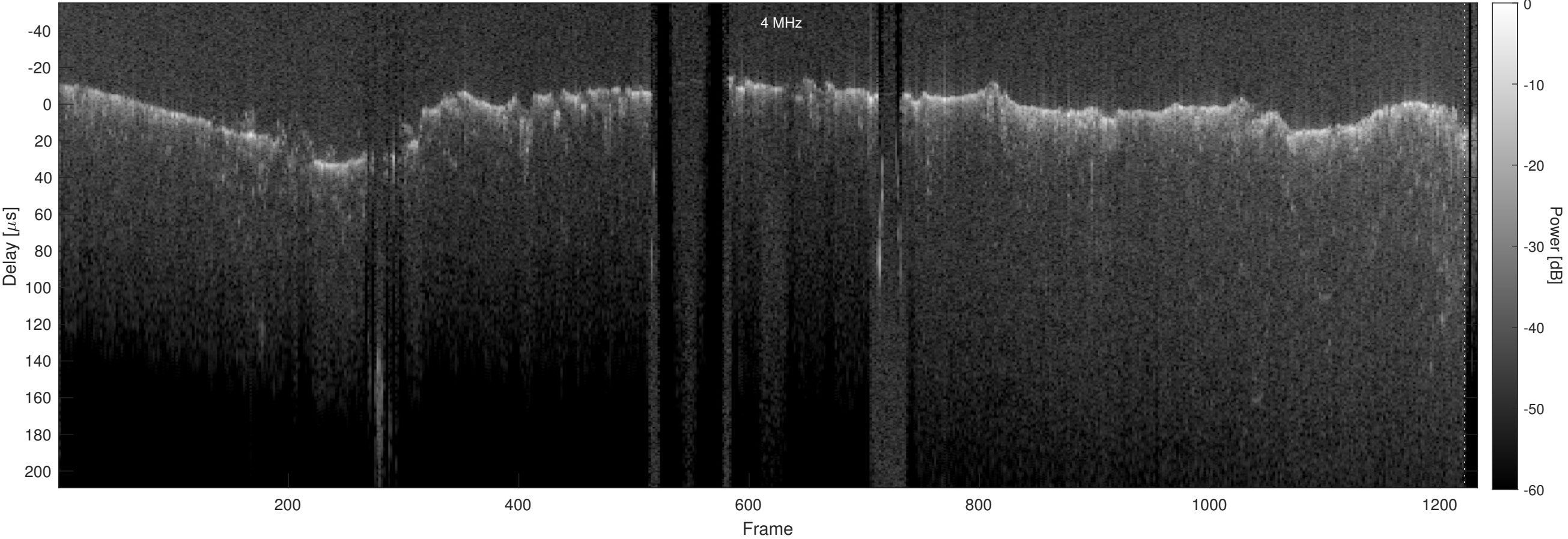
Orbit 4137, Optimized, No Window, Channel 2
